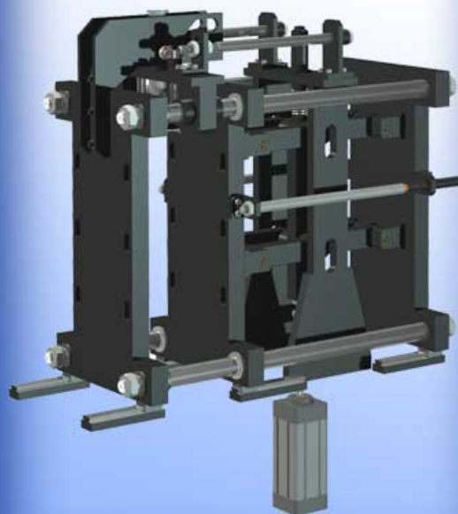
Clamping Unit
